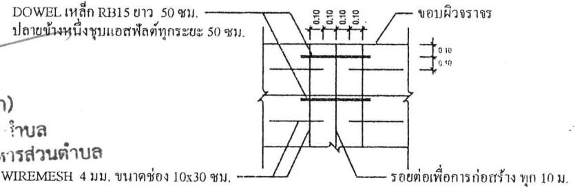
DETAIL (B)
